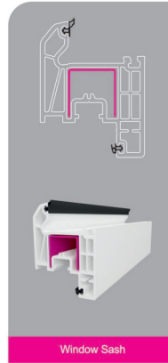
Window Sash
